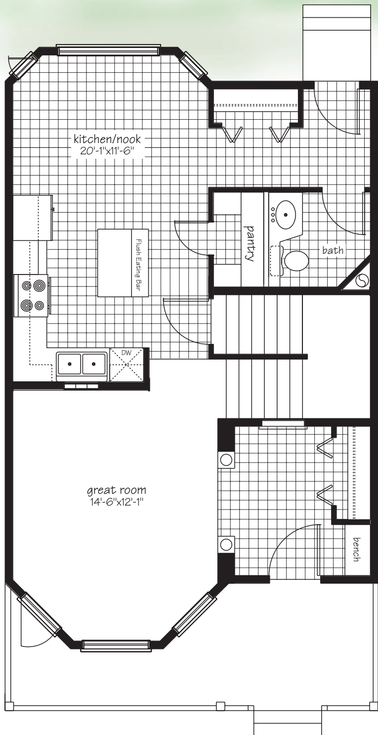
Main Floor Plan - 707 sq. ft.
