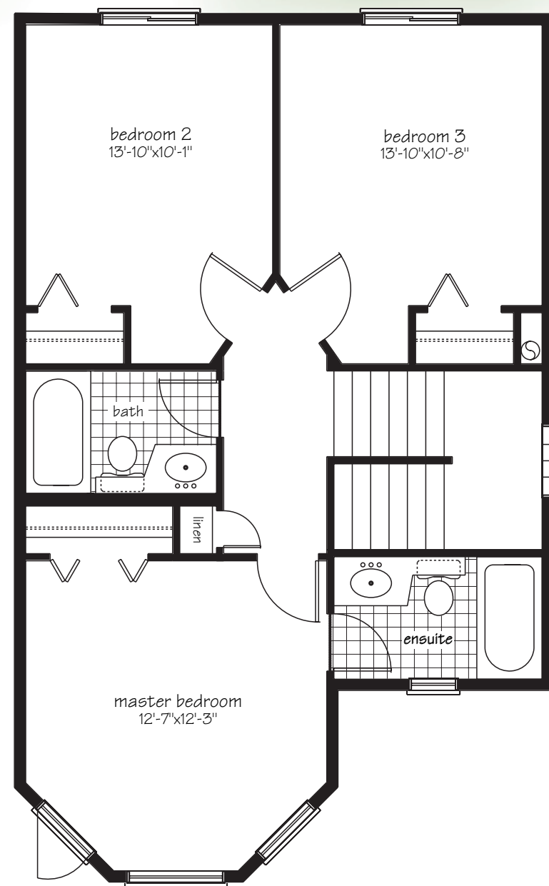
Upper Floor Plan - 631 sq. ft.
