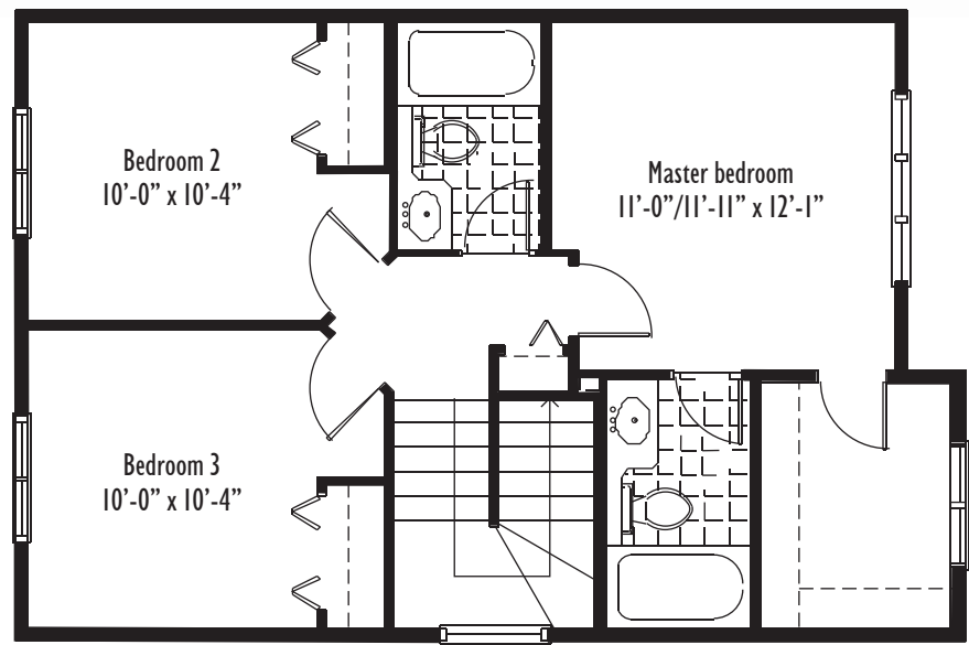
Upper Floor Plan - 642 sq. ft.
