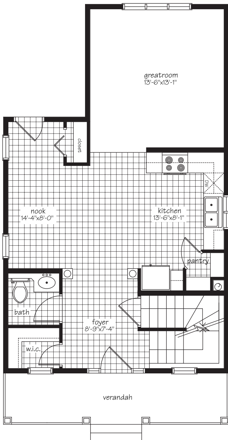
Main Floor Plan - 704 sq. ft.
