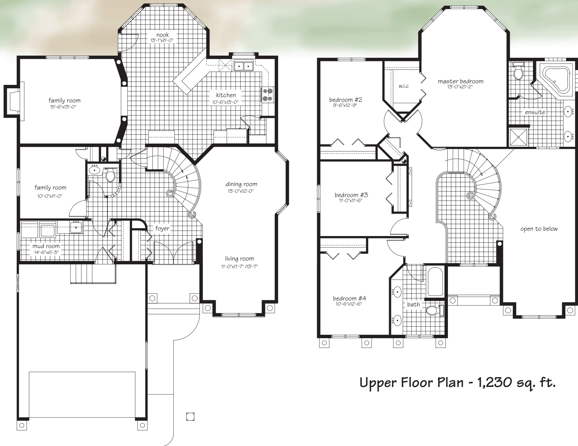
Main Floor Plan - 1,478 sq. ft.
