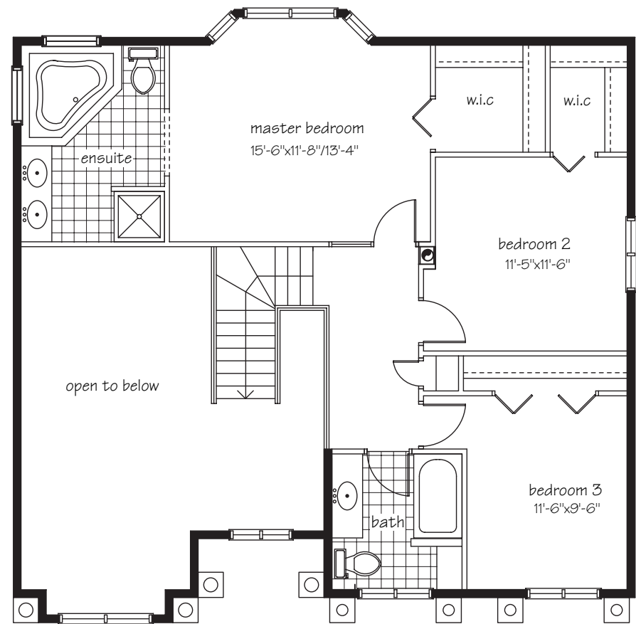
Upper Floor Plan - 853 sq. ft.
