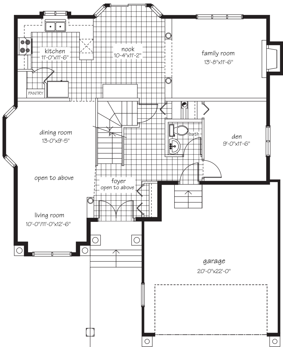
Main Floor Plan - 1,098 sq. ft.
